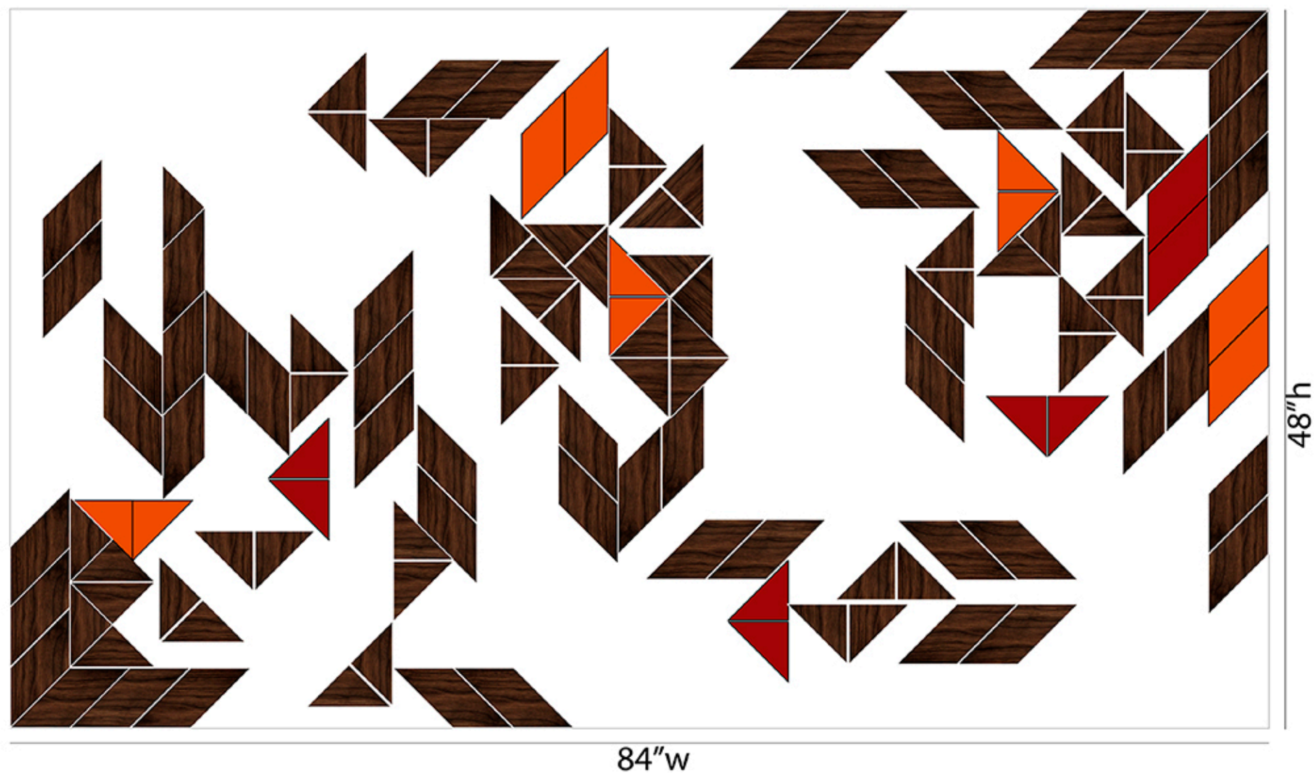
Geometric Wall Sculpture shop drawing
